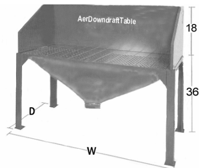
Above table shown with optional 18" high non-sparking aluminum side shields.
